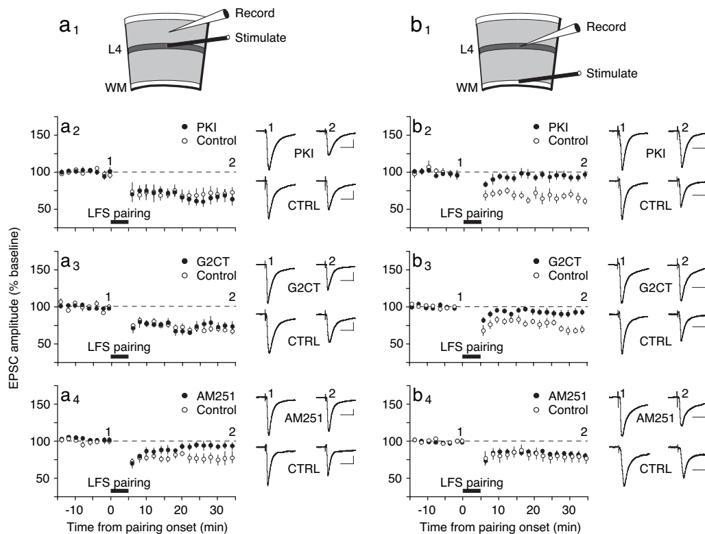
Fig. 3. Differences in pairing-induced LTD in layers 4 and 3 of visual cortex. ( a and b ) Displayed are grouped data time courses and representative sweeps from layers 2/3 ( a ) and 4 ( b ) recordings. LTD was challenged both extracellularly and intracellularly by a battery of antagonists, which highlight differences in LTD expression between layers. ( a 1 and b 1 ) Schematic illustrations of recording configurations for layers 2/3 ( a 1 ) and 4 ( b 1 ). ( a 2 and b 2 ) Intracellular loading of a PKA inhibitor PKI (6–22 amide, 10 \mu M) prevented LTD in layer 4 ( b 2 ) but not in layer 2/3 ( a 2 ). ( a 3 and b 3 ) Intracellular loading of G2CT (10 \mu M), a peptide that interferes with regulated endocytosis of GluR2, also prevents LTD in layer 4 ( b 3 ) but not layer 2/3 ( a 3 ). ( a 4 and b 4 ) Bath application of the CB1 antagonist AM251 (2 \mu M) had no effect on LTD in layer 4 ( b 4 ) but largely prevented LTD in layer 2/3 ( a 4 ). The y axis is EPSC amplitude normalized to a 15-min baseline period, with error bars indicating the SEM. The pairing protocol, denoted by the black bar, was administered at time 0 and lasted 5 min. The dashed horizontal line indicates no change from baseline responses. Sweep numbers (1 and 2) refer to averaged responses collected during the last 5 min of the baseline and postpairing periods. Stimulation artifacts were minimized for clarity. (Scale bars: 50 pA, 20 msec.) See Fig. 4 for statistical comparisons.
