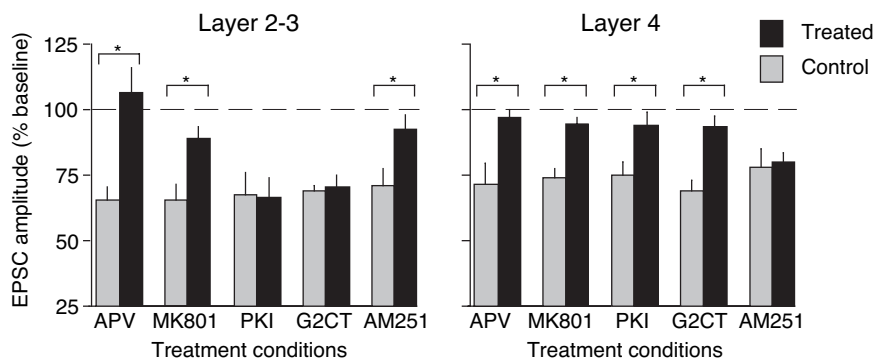
Fig. 4. Summary data comparing laminar differences in LTD. Filled bars represent mean \pm SEM of EPSC 25–30 min after LFS (normalized to baseline) in neurons treated with the drugs indicated. Gray bars represent the effect of LFS in the interleaved vehicle-treated controls. The number of experiments in each group is indicated in the text. Note the consistency of LTD magnitude in all control experiments. APV and AM251 were bath-applied. MK801, PKI, and G2CT were loaded intracellularly. *, P < 0.01 .
