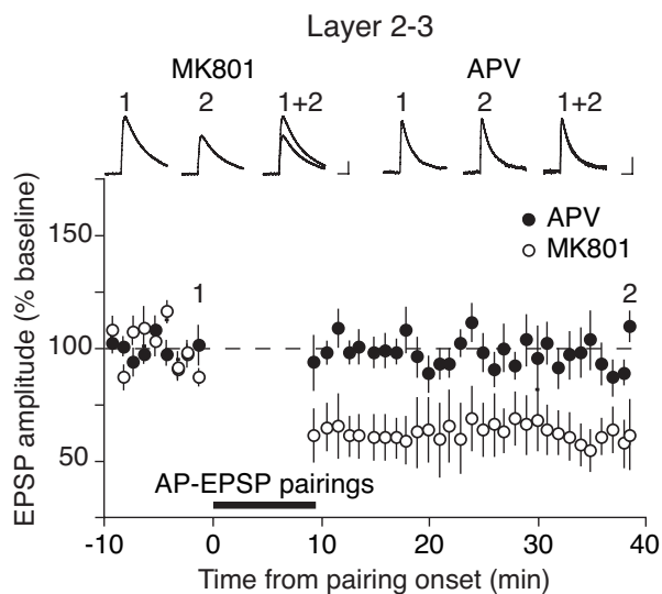
Fig. 2. Spike-timing LTD is insensitive to postsynaptic NMDAR blockade. Displayed are grouped data time courses and representative sweeps from whole-cell current-clamp recordings examining STD-LTD from visual cortex slices obtained from P13–P15 mice (15). In contrast to LFS-LTD, cells loaded with MK801 manifested robust STD-LTD (EPSP amplitude, 62.4 \pm 11.9\% ; slope, 62.4 \pm 15.3\% ; n = 7 ), whereas bath application of APV prevented STD-LTD (EPSP amplitude, 95.5 \pm 6.7\% ; slope, 99.1 \pm 13.9\% ; n = 7 ). 1 and 2 indicate 5-min periods for the averaging of EPSPs just before pairing (1) or at the conclusion of the recording session (2). Stimulus artifacts were minimized for clarity. (Scale bar: 1 mV, 10 msec.) The dashed line indicates no change from baseline responses.
