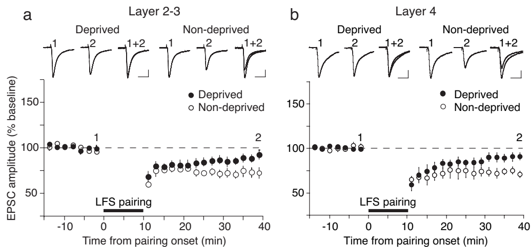
Fig. 5. Prior MD occludes subsequent LTD ex vivo in layers 2/3 and 4. (a and b) Male mice (P21–P28) were monocularly deprived for 3 days. On the third day, slices were obtained and whole-cell voltage-clamp recordings were performed from the binocular area of the deprived hemisphere (contralateral to the lid-sutured eye) or from the control hemisphere (ipsilateral to the lid-sutured eye). LTD was saturated by doubling the LFS-pairing protocol duration to 10 min. In both layers, robust LTD was induced in the control nondeprived hemisphere (a, layer 2/3, 73.8 \pm 5.4\% , n = 6 ; b, layer 4, 72.6 \pm 3.3\% , n = 5 ). In contrast, LTD was significantly occluded in the deprived hemisphere (a, layer 2/3, 89.5 \pm 3.6\% , n = 7 , P < 0.05 ; b, layer 4, 90.1 \pm 3.6\% , n = 6 , P < 0.01 ). 1 and 2 indicate 5-min periods for the averaging of EPSCs just before pairing (1) or at the conclusion of the recording session (2). Stimulus artifacts were minimized for clarity. (Scale bars: 50 pA, 20 msec.) The dashed line indicates no change from baseline responses. Recordings were performed with the experimenter blind to the visual history of the animal.
